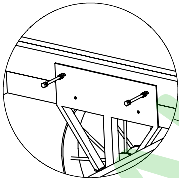
bolt M10x110
