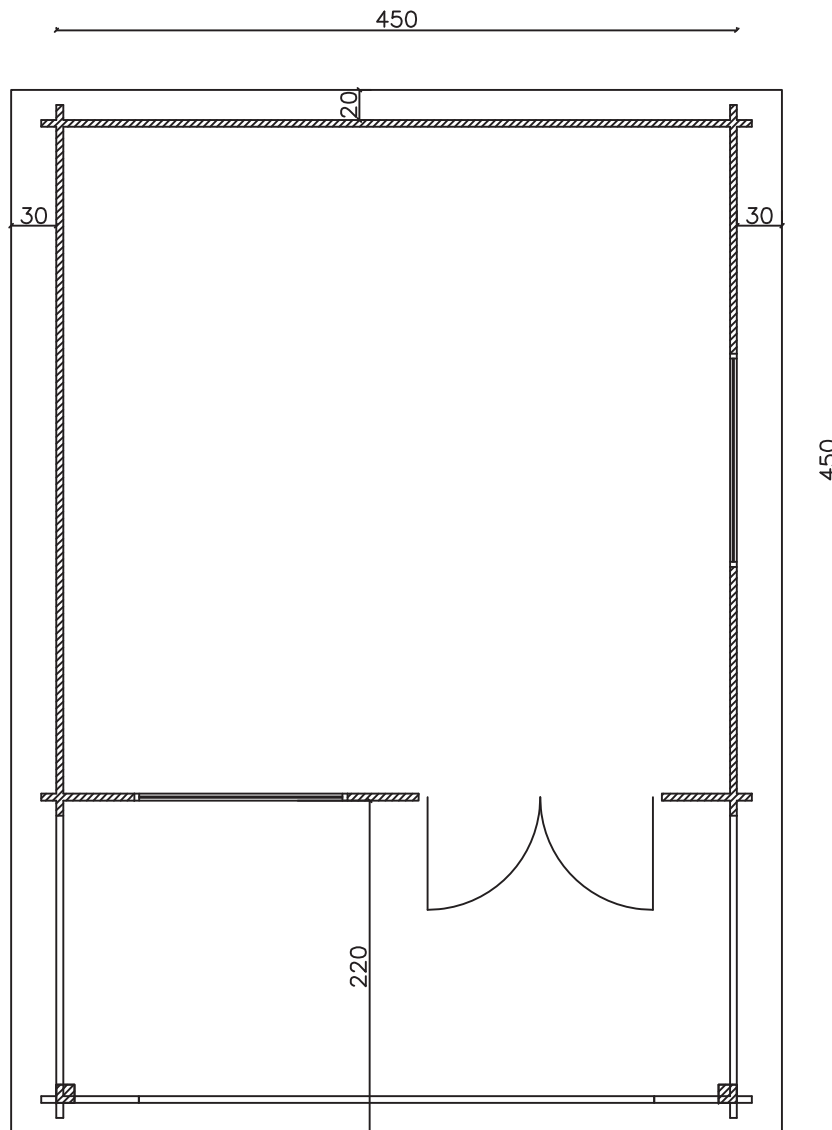
Grundriss / ground plan / plattegrond / plan / rzut
