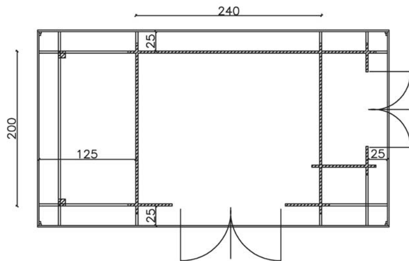
Grundriss / ground plan plattegrond / plan / rzut
